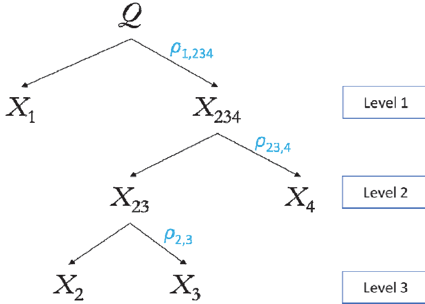
Figure 6. Example of nested CES function with 4 inputs
