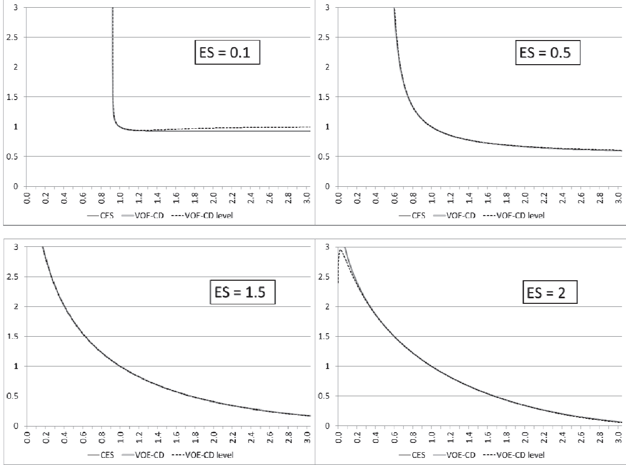
Figure 1. Isoquant for various ES
