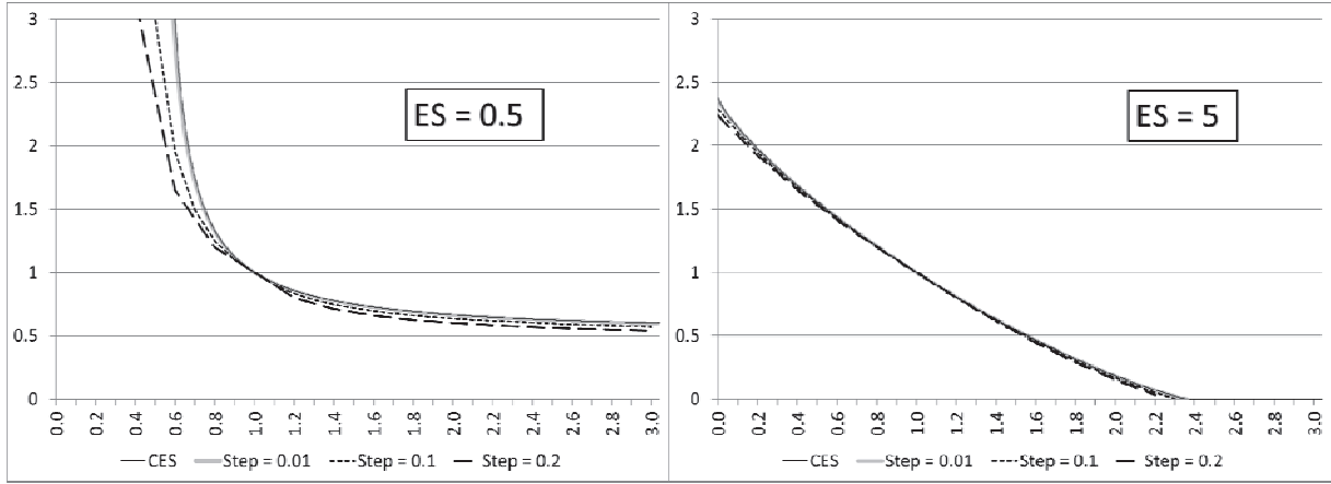
Figure 2. Isoquant for various steps
